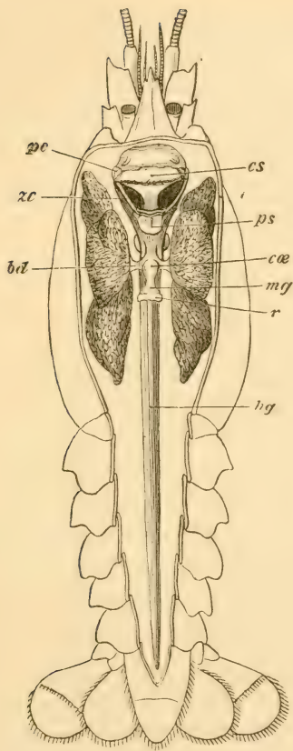
FIG. 13.— Astacus fluviatilis .—The alimentary canal and livers seen from above (nat. size). bd , bile-duct; ca , caecum; es , cardiac portion of stomach, the line pointing to the cardiac ossicle; hg , hind-gut; mg , mid-gut; pc , pterocardiac ossicle; ps , pyloric portion of stomach, the line pointing to the pyloric ossicle; r , ridge separating mid-gut from hind-gut; zc , zygocardiac ossicle.
